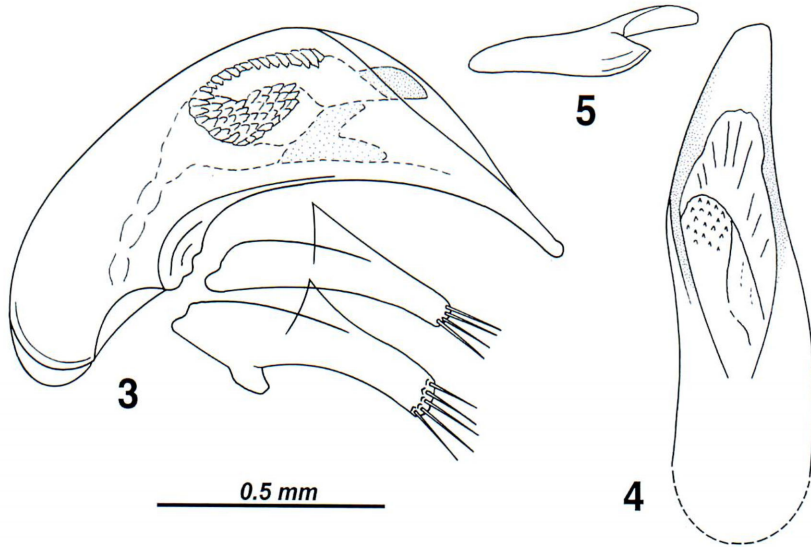
Figs. 3–5. Male genitalia of Trechiamia (s. str.) ion ASHIDA et SOUMA, from Taniguchi in Takebe-chô; left lateral (3) and dorsal (4) views, and separated copulatory piece, left lateral view (5).
