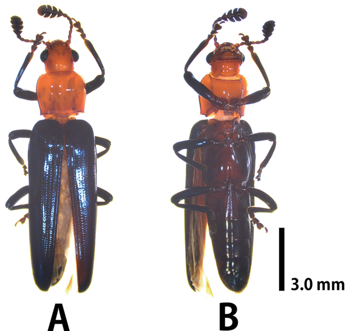
Fig. 1. Caenolanguria azurea VILLIERS. ——— A, Dorsal view; B, ventral view.
